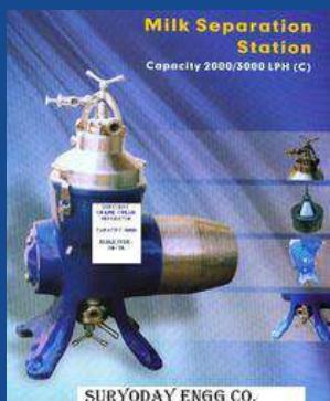
Online Cream Separator 3000 LPH
